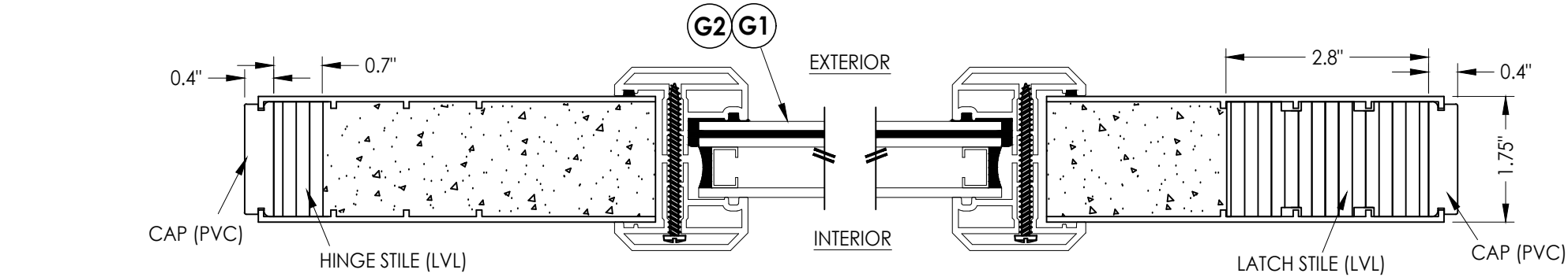
1 3 HORIZONTAL CROSS SECTION
